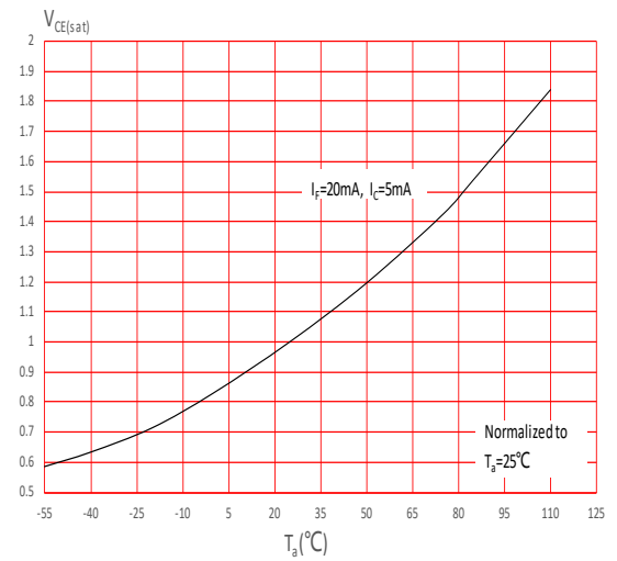
FIG.8: Normalized Collector-emitter Saturation Voltage vs. Ambient Temperature
