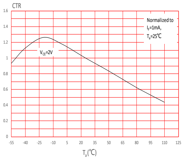
FIG.7: Normalized Current Transfer Ratio vs. Ambient Temperature
