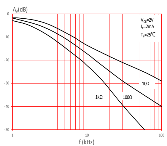
FIG.10: Frequency Response
